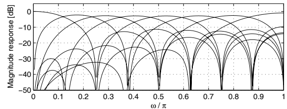
Fig. 6. Magnitude response of DCT approximation based on the CORDIC algorithm.
