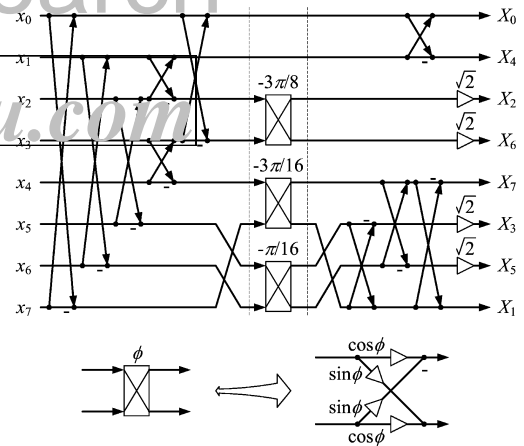
Fig. 1. Signal flow graph of Loeffler's factorization [2] of the eight point DCT.
