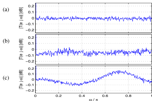
Fig. 8. Sum of squared magnitude responses using lattice (a), CORDIC (b) and binDCT-L3 (c).
