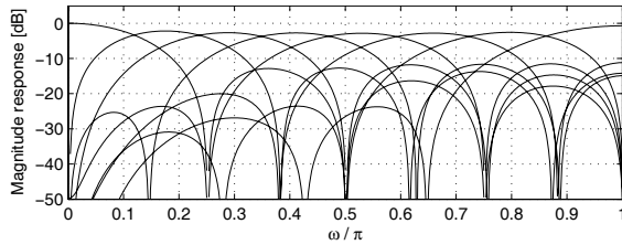
Fig. 4. Magnitude response of DCT approximation based on coefficients in Table 2 ( \tan \beta \approx -9/32 ).
